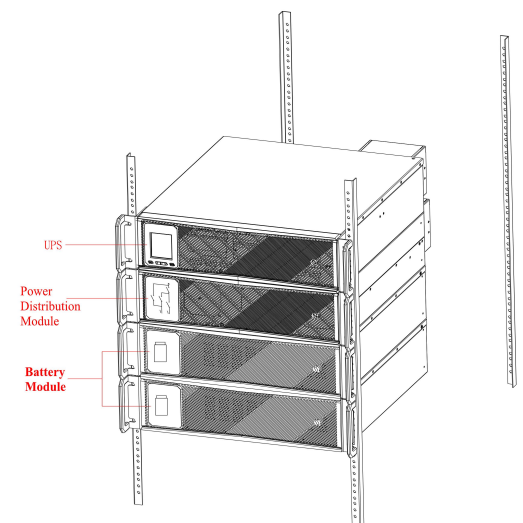
* Rack-mounted UPS Installation with Distribution Module and Battery Module
